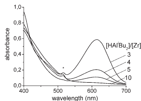
Figure 5. UV/vis absorption spectra of toluene solutions containing 0.56 mM (\text{SBI})\text{ZrCl}_2 in the presence of 3, 4, 5, or 10 equiv of \text{HAl}^i\text{Bu}_2 , after addition of 1 equiv of [\text{Ph}_3\text{C}][\text{B}(\text{C}_6\text{F}_5)_4] (path length 1 cm; *artifact due to change of gratings).
