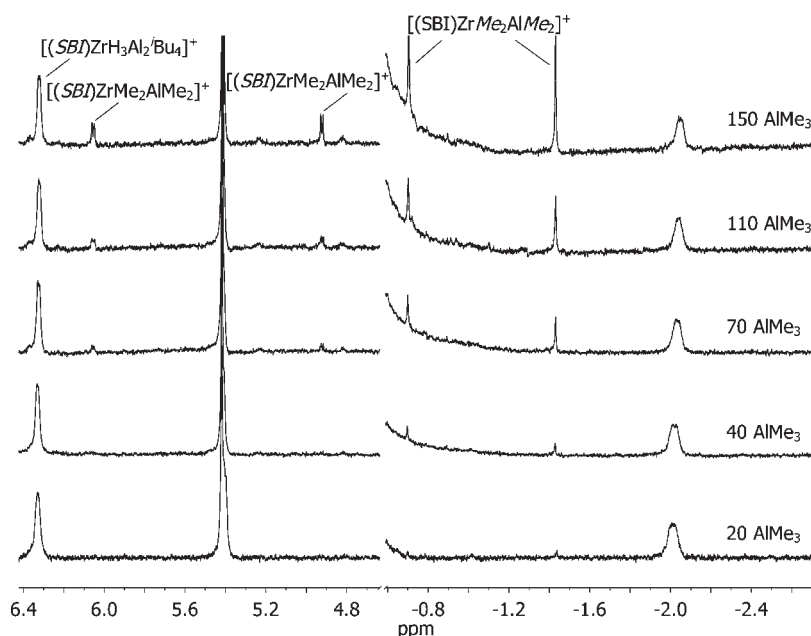
Figure 7. ^1\text{H} NMR spectra of a 3 mM solution of [(\text{SBI})\text{Zr}(\mu\text{-H})_3(\text{Al}^i\text{Bu}_2)_2]^+ with 3.5 equiv of free \text{HAl}^i\text{Bu}_2 in benzene- d_6 , upon addition of 20–150 equiv of \text{AlMe}_3 relative to Zr.
