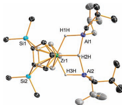
Figure 4. Structure of the cation [(\text{Me}_2\text{Si})_2(\text{C}_5\text{H}_3)_2\text{Zr}(\mu\text{-H})_3(\text{Al}^i\text{Bu}_2)_2]^+ in crystals of its [\text{B}(\text{C}_6\text{F}_5)_4]^- salt (thermal ellipsoids drawn at 50% probability, hydride positions taken from the difference Fourier map; other H atoms omitted).
