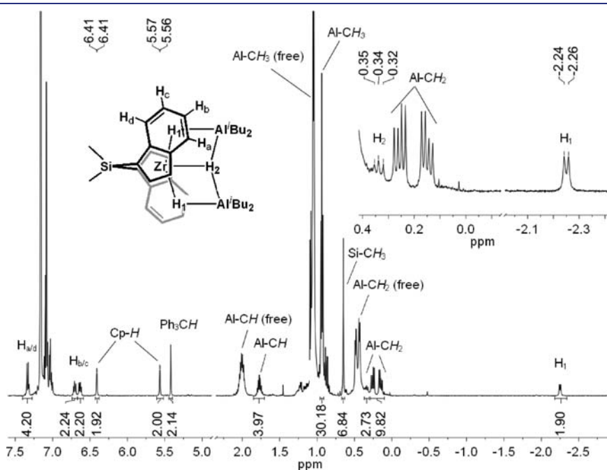
Figure 1. 1 H NMR spectrum of the cationic hydride [(SBI)Zr( μ -H) 3 (Al i Bu 2 ) 2 ] + in benzene- d 6 solution, obtained by treating a 4 mM solution of (SBI)ZrCl 2 first with 5 equiv of HAl i Bu 2 and then with 1 equiv of [Ph 3 C][B(C 6 F 5 ) 4 ] (25 °C, 500 MHz).
